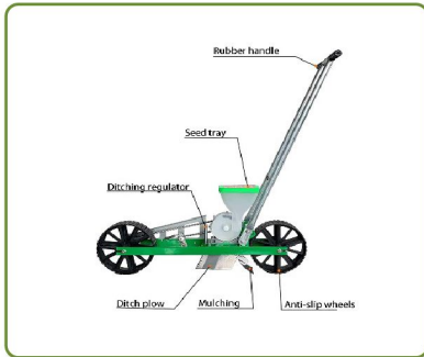
Single Row Hand Push Small Manual Seeder
